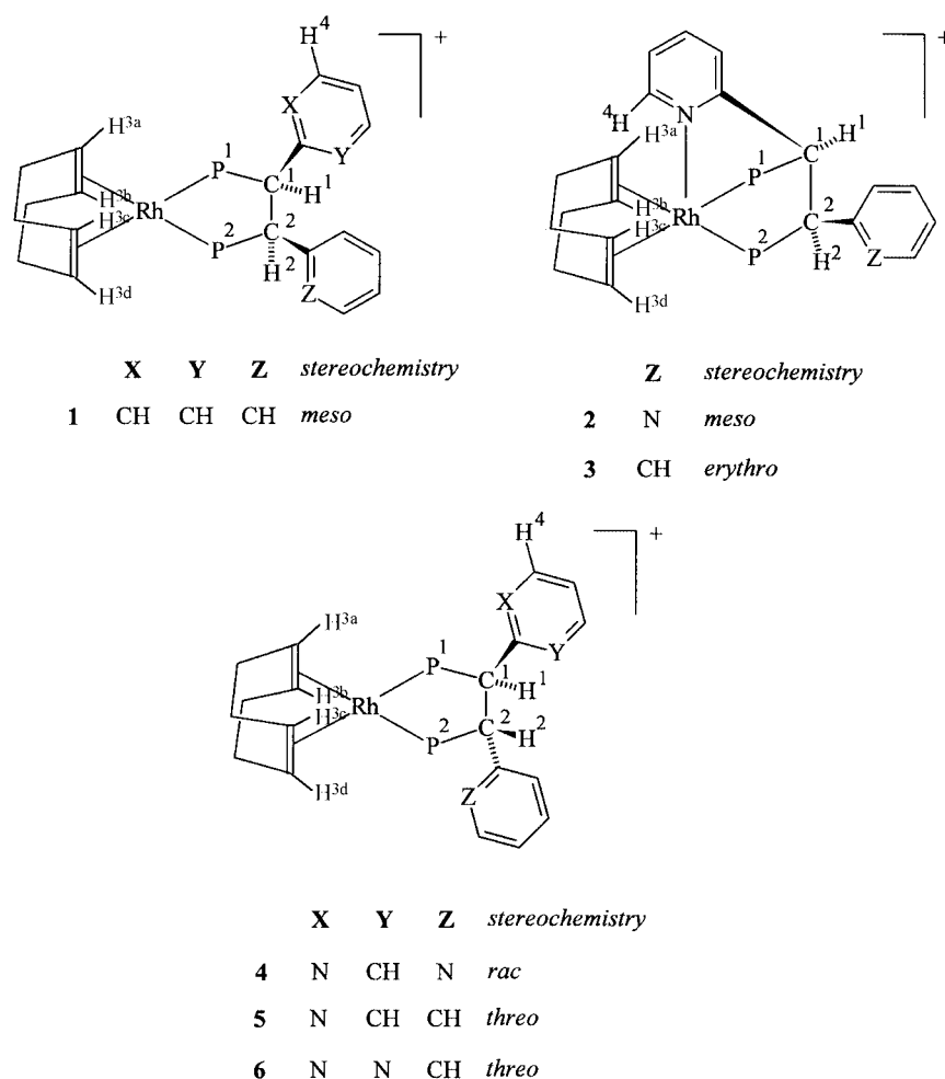
Fig. 1 Schematic structures and partial NMR labelling system for the cations of 1–6 . Phenyl groups on the phosphorus atoms have been omitted for clarity. 'Stereochemistry' refers to that of the parent ligand (before coordination). The relative assignment of H 3a –H 3d is arbitrary.
