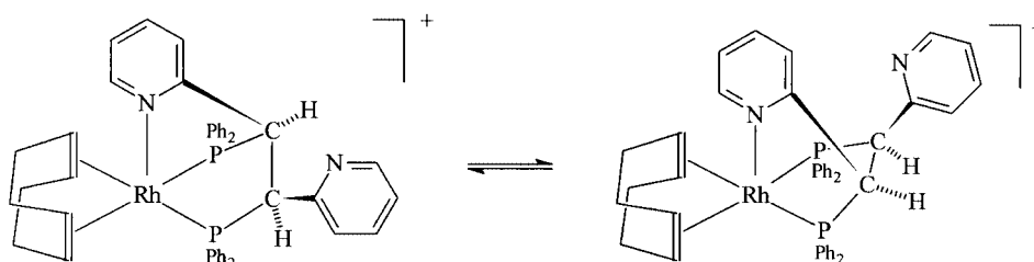
Fig. 2 Representation of the fluxional behaviour available to compound 2 .
